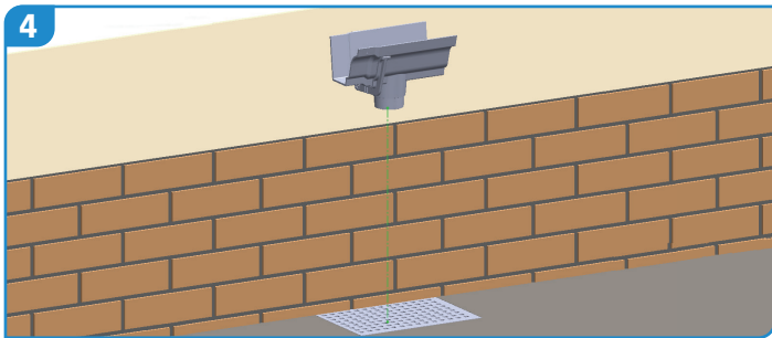
4 With the use of a plumb or laser line, position outlets over gullies and support with at least one bracket. Also include a bracket per angle (internal or external).
